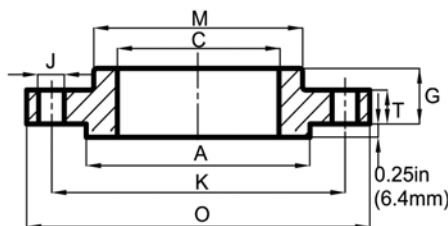
SLIP-ON
