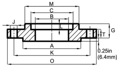
SOCKET WELDING
