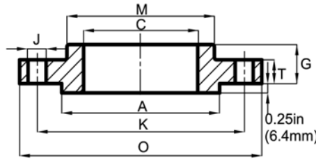
SLIP-ON
