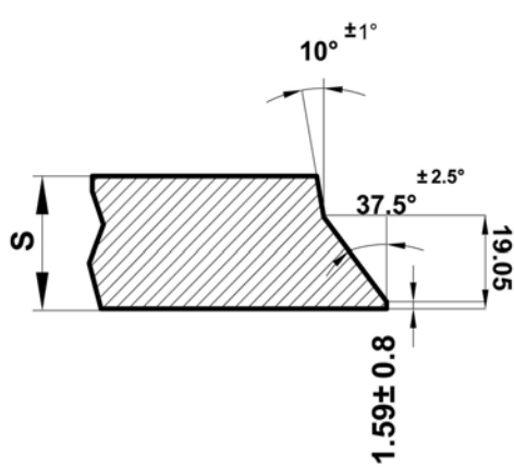
Compound Bevel
