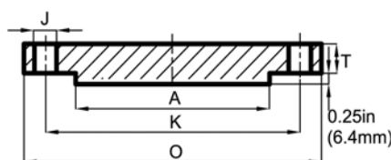
BLIND
