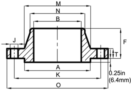
WELDING NECK
