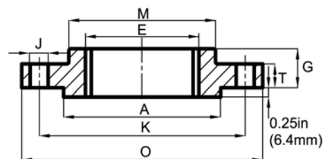
THREADED
