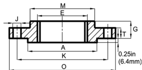
THREADED
