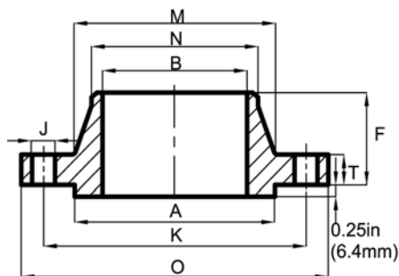
WELDING NECK
