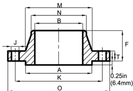
WELDING NECK
