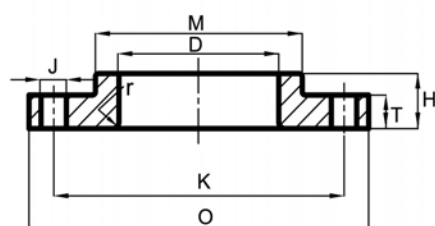
LAP JOINT
