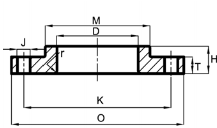
LAP JOINT
